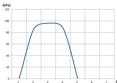
Chart of pressure rise inside a 32 mm diameter air button (such as the 66ZM5 model described in this catalog)
